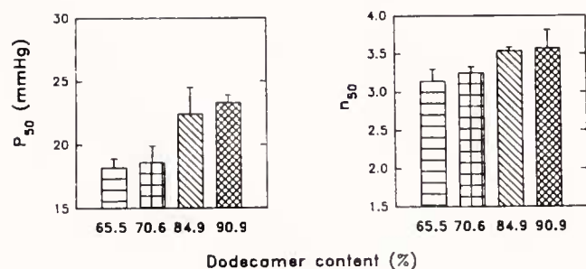
Figure 4. O 2 binding properties (cell respiration procedure) of native Hcs with different contents of dodecamers. 25°C, pH 7.50. Buffered saline as in Figure 1. Mean \pm S.E. ( n = 6 ).
